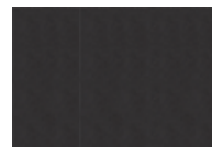
Graphite
