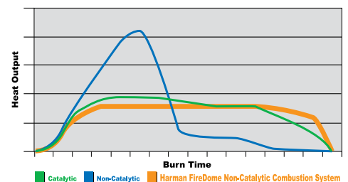
Typical Low Burn Rate Patterns for Three Basic Types of Wood-Burning Stoves
